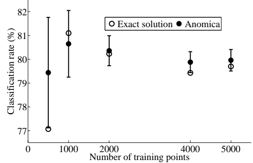
Figure 5. Figure comparing the classification rate of the test set using classical one class SVMs and \nu -Anomica algorithm with different sizes of the training sets using OPAD data.
