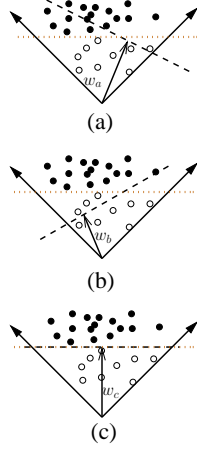
Figure 2. This figure shows the update rules of \nu -Anomica. Subfigures (a) and (b) represent the over classified and under classified cases respectively. In subfigure (c) the evaluated classification rate of the current model meets the “ \nu -criterion”. The target hyperplane and the current hyperplane is represented by dotted and dashed line respectively.
